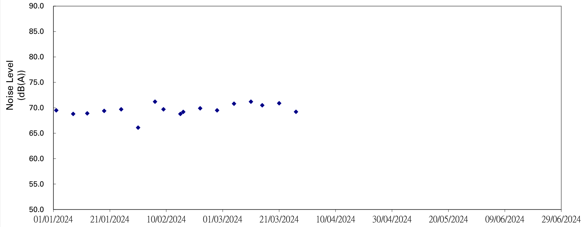
Noise Level (Leq 30 mins) dB(A) Vs Date for Location W-N18
